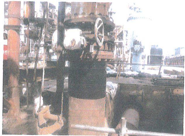
② First, two technicians from ORIHARA and one person from the contractor start the work jointly. As pre-treatment, apply BUTYL ROLL over the pipe to even out its surface.
